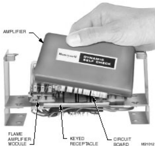
Fig. 2. Mounting the R7476A,B Amplifier on the Flame Safeguard Control.
